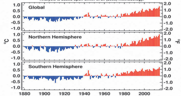
June Land & Ocean Surface Mean Temp Anomalies NCEP/NESDIS/NOAA Analysis is based upon Smith et al. (2008) methodology.
